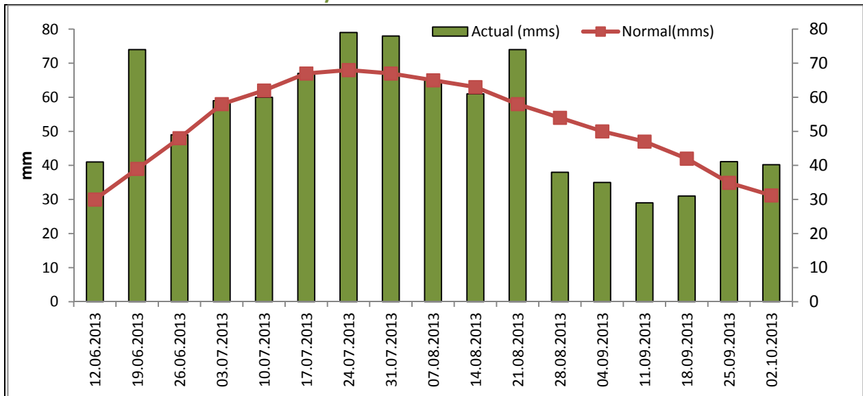
Chart 5: Trends in Weekly Rainfall Distribution in Monsoon 2013-All India
