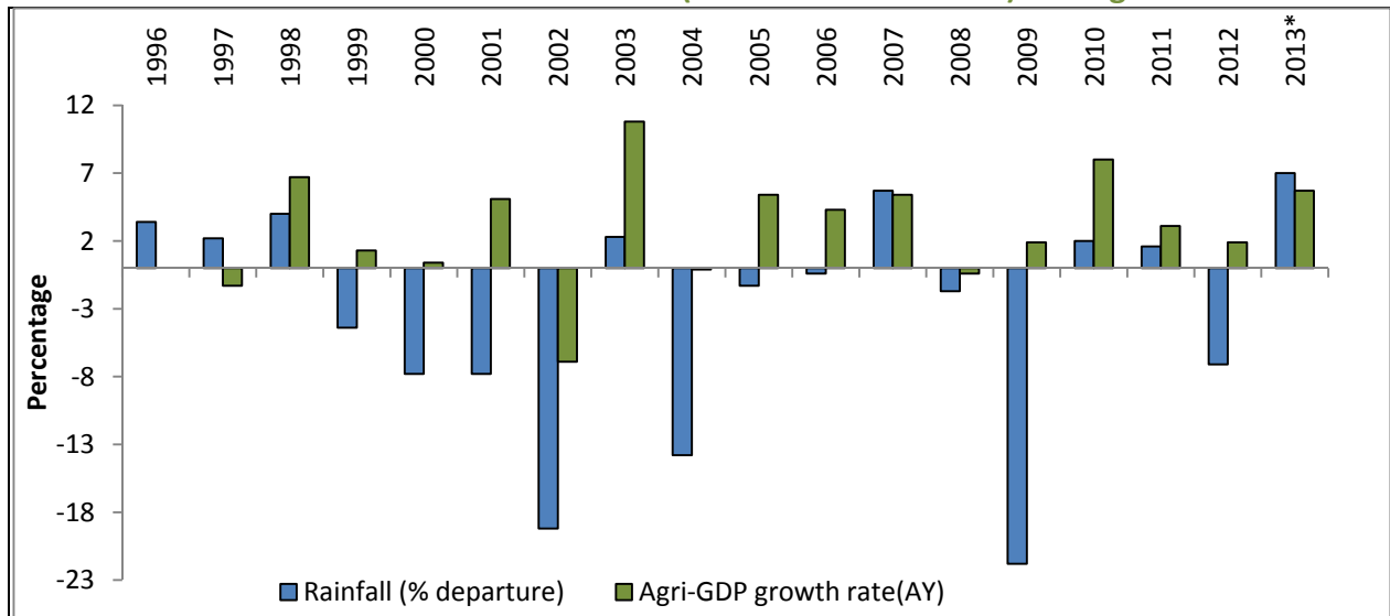
Chart 6: Co-movements of Rainfall (% deviation from LPA) and Agri-GDP
