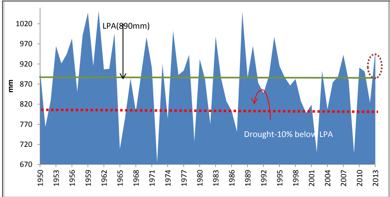
Chart 3: Trend in Indian Monsoon Rains
